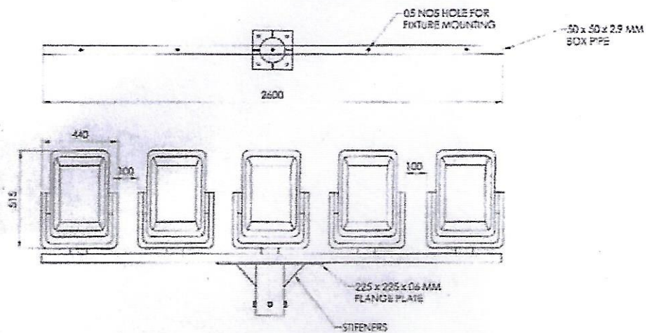
BRACKET FOR 5 NOS. OF FLOOD LIGHT FIXTURES
