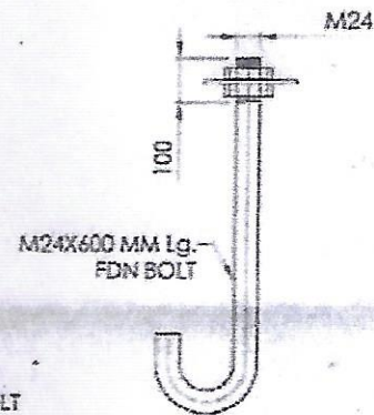
FOUNDATION BOLT
