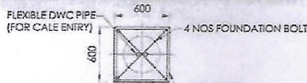
FOUNDATION TOP VIEW
