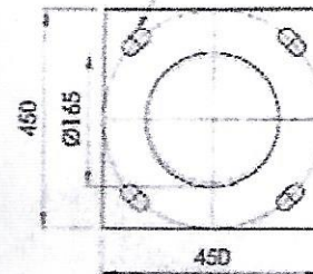
BASE PLATE 450X450X16
