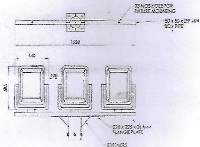
BRACKET FOR 3 NOS. OF FLOOD LIGHT FIXTURES
