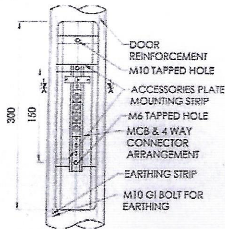
DOOR DETAIL DETAIL-'A'
