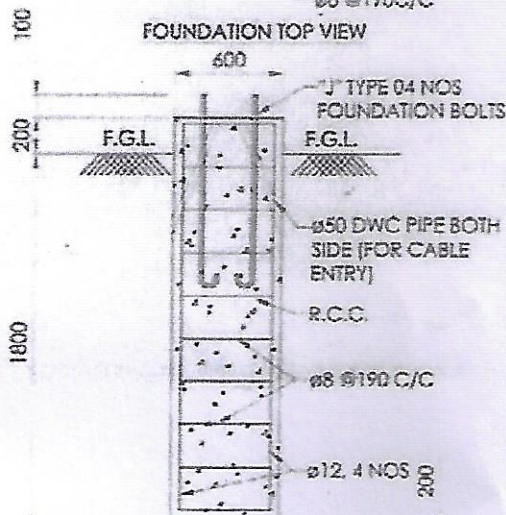
FOUNDATION DETAILS
