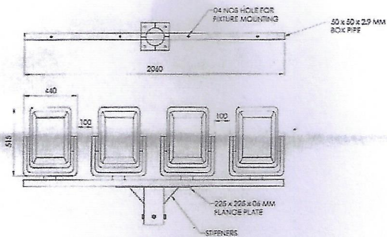
BRACKET FOR 4 NOS. OF FLOOD LIGHT FIXTURES
